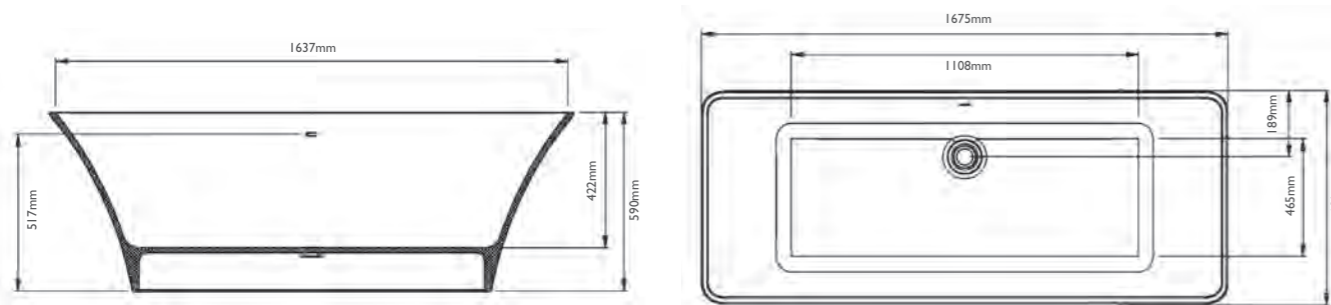
Dimensions can differ +/- 5%
