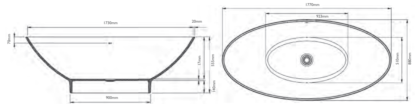
Dimensions can differ +/- 5%
