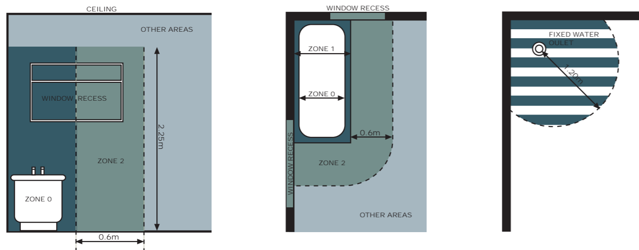
Elevation view of bath tub
