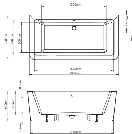
Wall-Mounted version (to go against the wall)
